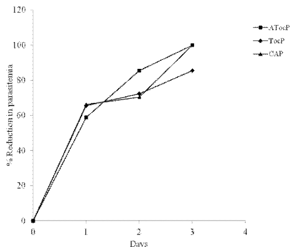
Figure 1: % Reduction in Parasitemia showing the effect of Aqueous Extract of T. occidentalis on Artesunate in P.berghei berghei infected mice.
