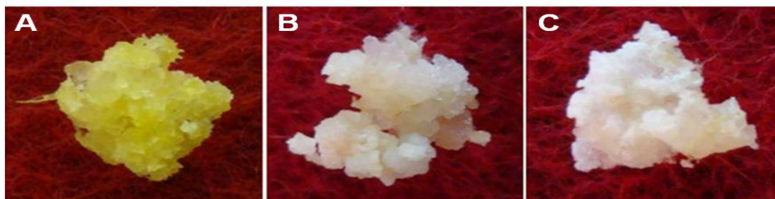
Figure 1. Different types of callus of tall fescue. A, Embryogenic callus (+++++); B and C represents the non-embryogenic type (+++) of callus of Greenmaster variety, respectively. + = Poor, +++ = Average, +++++ = Best.
