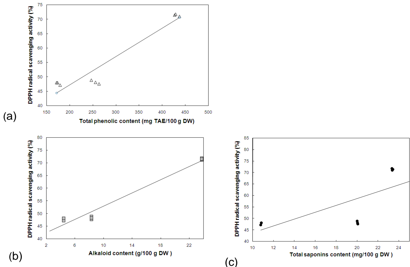
Figure 2. Correlations between phytochemical content and DPPH scavenging activity for (a) total phenolic ( \Delta ); (b) alkaloid ( \square ) and (c) total saponins ( \bullet ) content (n=9, Pearson coefficient of 0.95, 0.98 and 0.72, respectively at p < 0.01 ).
