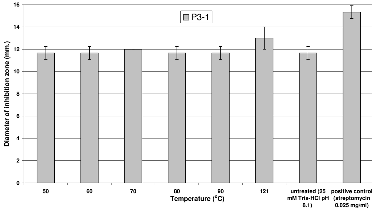
Figure 5. Inhibition zone against B. cereus ATCC 11778 of P3-1 after treatment with high temperatures compared with untreated protein. The antimicrobial activity of P3-1 against B. cereus ATCC 11778 was tested after treating P1 at high temperatures of 50, 60, 70, 80 and 90°C for 60 min and 121°C for 30 min. The clear zones of inhibition were measured for their diameter. Values represent the mean \pm SD for three replicates.
