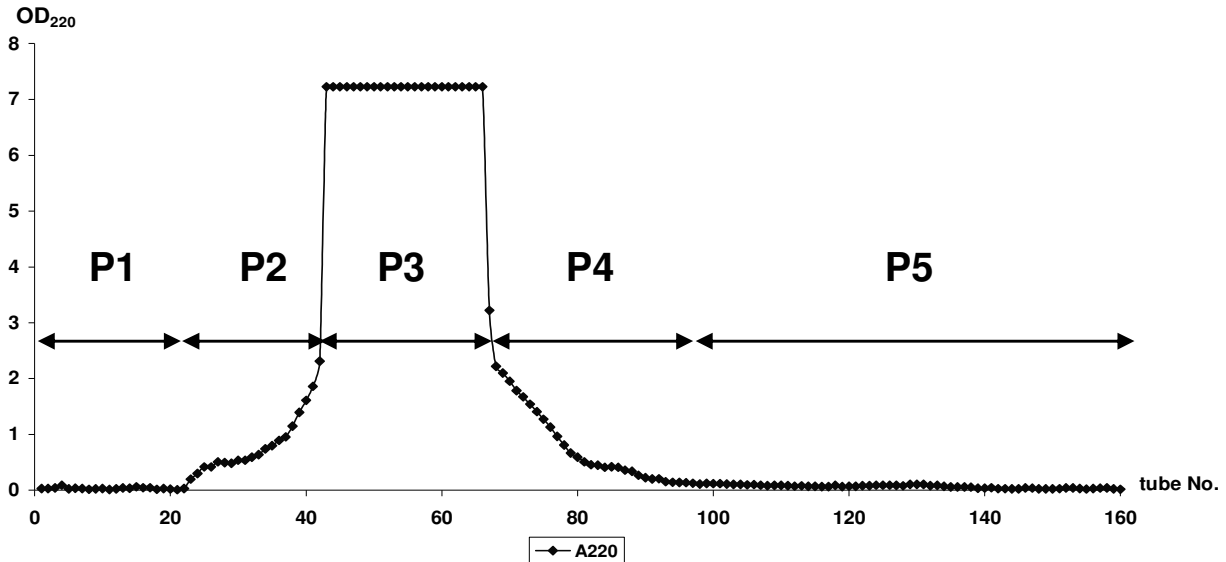
Figure 2. Elution profile of evaporated culture filtrate from Streptomyces sp. No. 87 after purification by gel filtration chromatography with a sephadex G-25 resin column at 220 nm. The chromatogram at the absorbance of 220 nm (A220) was obtained after purification by gel filtration chromatography with a sephadex G-25 resin column. Flow rate was 1.00 ml/min and 5 ml/fraction was used.
