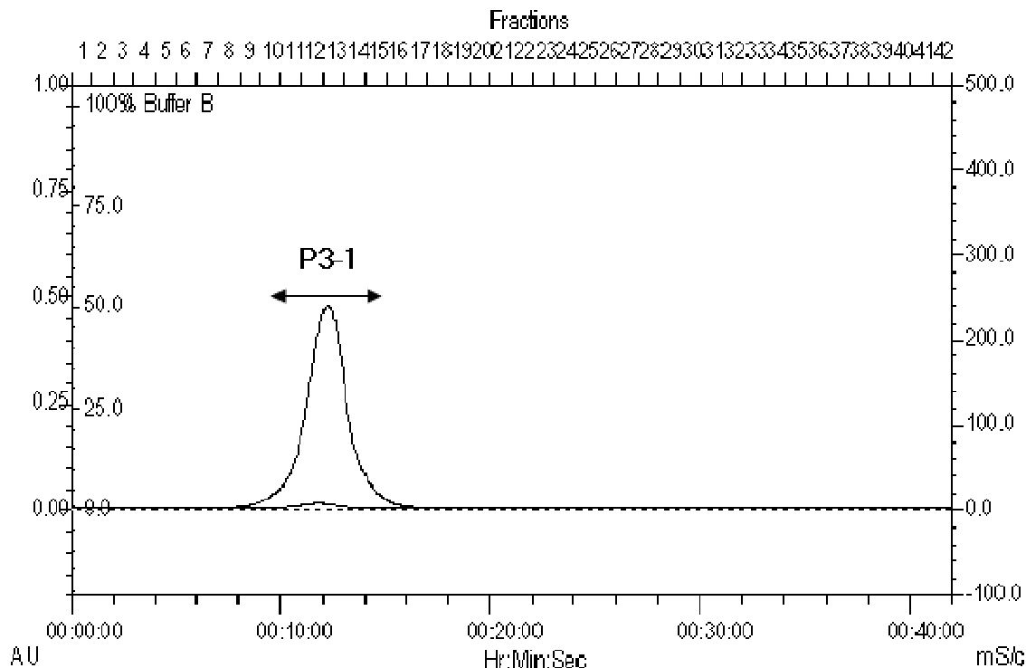
Figure 3. The elution profile of P3-1 from evaporated culture filtrate Streptomyces sp. No. 87 after purification through fast performance liquid chromatography (FPLC) with a superdex 30 column. The antimicrobial activity peaks from gel filtration chromatography were diluted with buffer A (25 mM pH 8.1 Tris-HCl buffer) (1:5, v/v). The diluent was filtrated through a 0.45 µm filter membrane and fractionated by FPLC with a sephadex 30 column. The pooled fractions which peaked at 280 nm were concentrated by evaporator.
