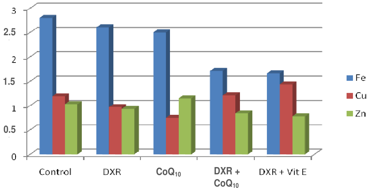
Figure 2. Comparison of trace element (Fe, Cu and Zn) levels in serum samples of the control, DXR, CoQ 10 , DXR + CoQ 10 and DXR + vitamin E groups.
