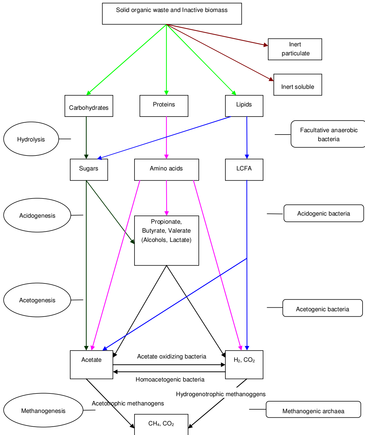
Figure 1. Main steps and pathways of dry anaerobic digestion process (modified from Batstone et al., 2002).
