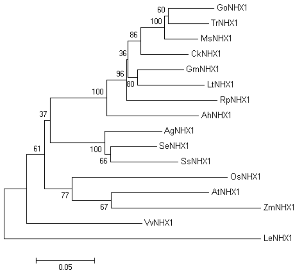
Figure 3. Phylogenetic tree of AhNHX1 amino acid and other plant species. AtNHX1 (AY685183), Arabidopsis Thaliana ; ZmNHX1 (AY270036); Zea mays ; OsNHX1 (AY324877), Oryza sativa ; AhNHX1 (HM590627), Arachis hypogaea ; GoNHX1 (EU340284), Galega orientalis ; TrNHX1 (EU109427), Trifolium repens ; CkNHX1 (DQ812099), Caragana korshinskii ; GmNHX1 (AY972078), Glycine max ; LtNHX1 (EU727217), Lotus tenuis ; RpNHX1 (EF675631), Robinia pseudoacacia ; VvNHX1 (AY634283), Vitis vinifera ; SsNHX1 (AF370358), Suaeda salsa ; SeNHX1 (AY131235), Salicornia europaea ; AgNHX1 (AB038492), Atriplex gmelini ; LeNHX1 (AJ306630), Lycopersicon esculentum ; MsNHX1 (GU265772), Medicago sativa .
