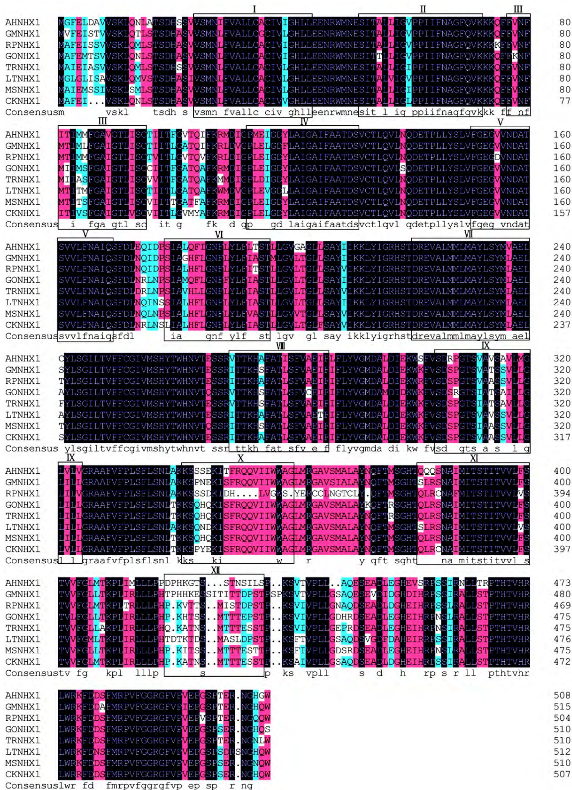
Figure 2. Comparison of AhNHX1 with other plants amino acid sequences of \text{Na}^+/\text{H}^+ antiporters and the predicted transmembrane of AhNHX1 protein. AhNHX1 (HM590627), Arachis hypogaea ; GmNHX1 (AY972078), Glycine max ; RpnHX1 (EF675631), Robinia pseudoacacia ; GonHX1 (EU340284), Galega orientalis ; TrnHX1 (EU109427), Trifolium repens ; LtNHX1 (EU727217), Lotus tenuis ; MsNHX1 (GU265772), Medicago sativa ; CknHX1 (DQ812099), Caragana korshinskii .
