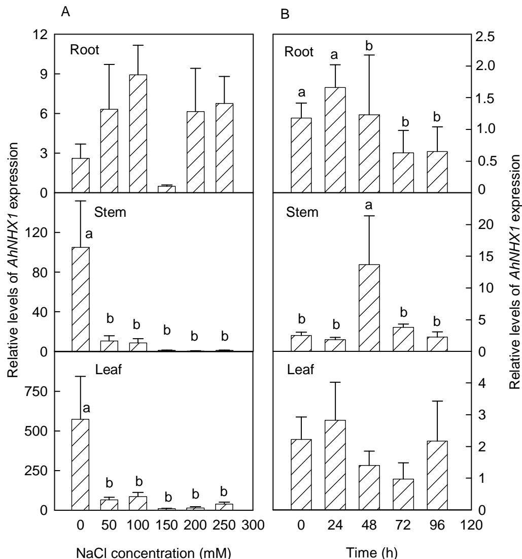
Figure 4. Real time RT-PCR analysis of the AhNHX1 gene under NaCl stress condition. A, Different NaCl concentration stress for 72 h; B, 150 mM NaCl stress for different time. Bars with different small or capital letters are significantly different at P < 0.05 or 0.01 .
