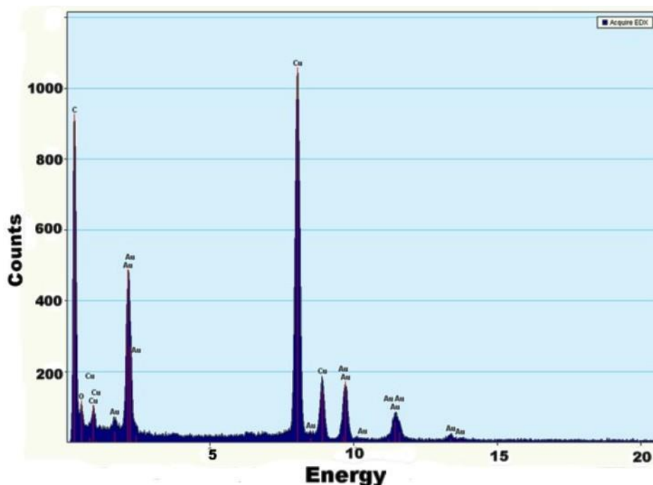
Figure 5: EDAX spectra of functionalized Polyethylene - AuNP with Lincomycin
