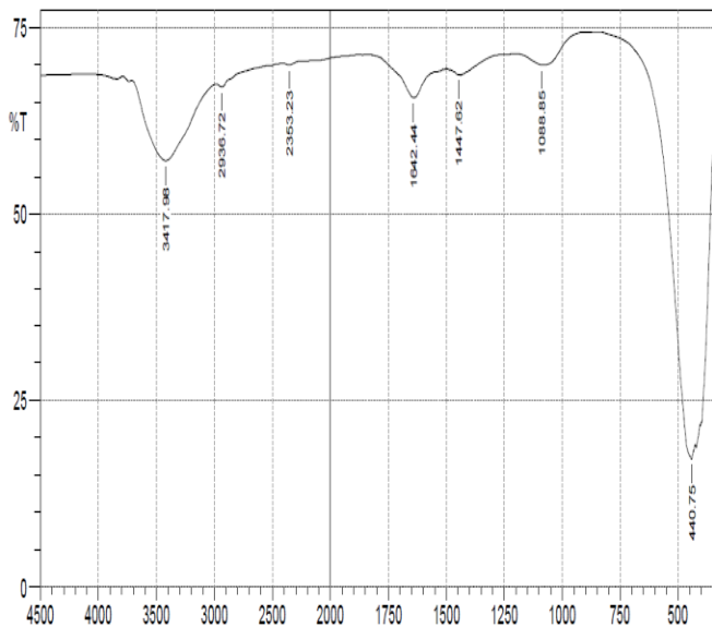
Figure 6: FTIR spectra of Catharanthus roseus extract capped Gold nanoparticle
