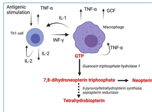
Figure 1: The synthesis of neopterin
