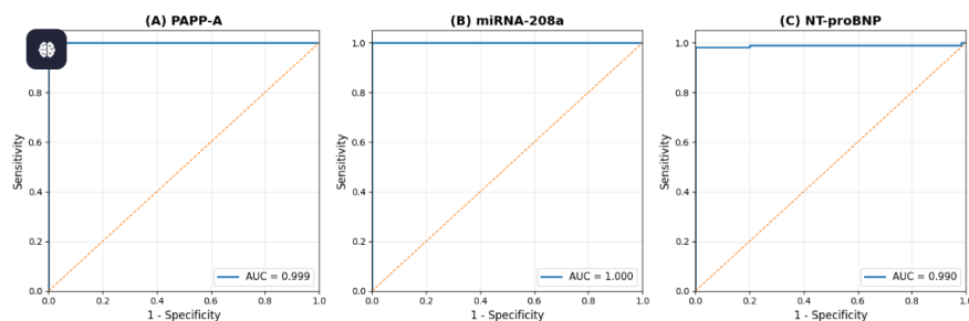
Figure 2: Receiver operating characteristic (ROC) curves for (A) PAPP-A, (B) miRNA-208a, and (C) NT-proBNP
