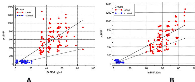
Figure 1: Scatter plots showing the relationship between (A) PAPP-A and NT-proBNP, and (B) miRNA-208a and NT-proBNP
