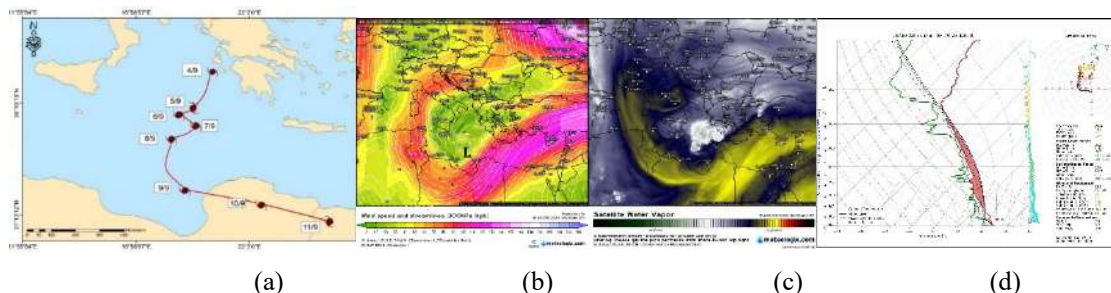
FIGURE 7 Storm track (a) jet stream axis penetration (b) water vapor mass (c) Skew-T thermodynamic chart 6.9.2023(Athens station)
