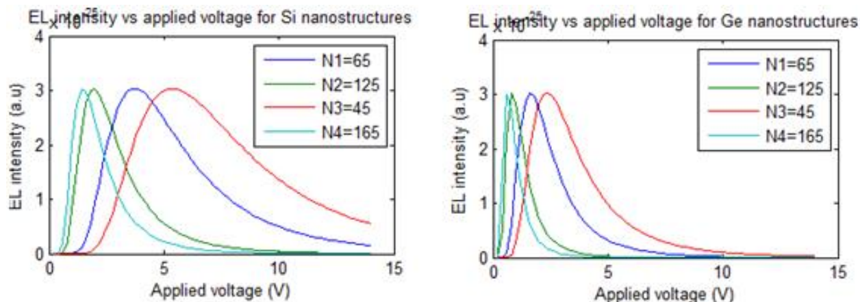
Figure 3: EL intensity as a function of applied voltage: the left graph is for Si nanostructures and the right one for Ge nanostructures.
