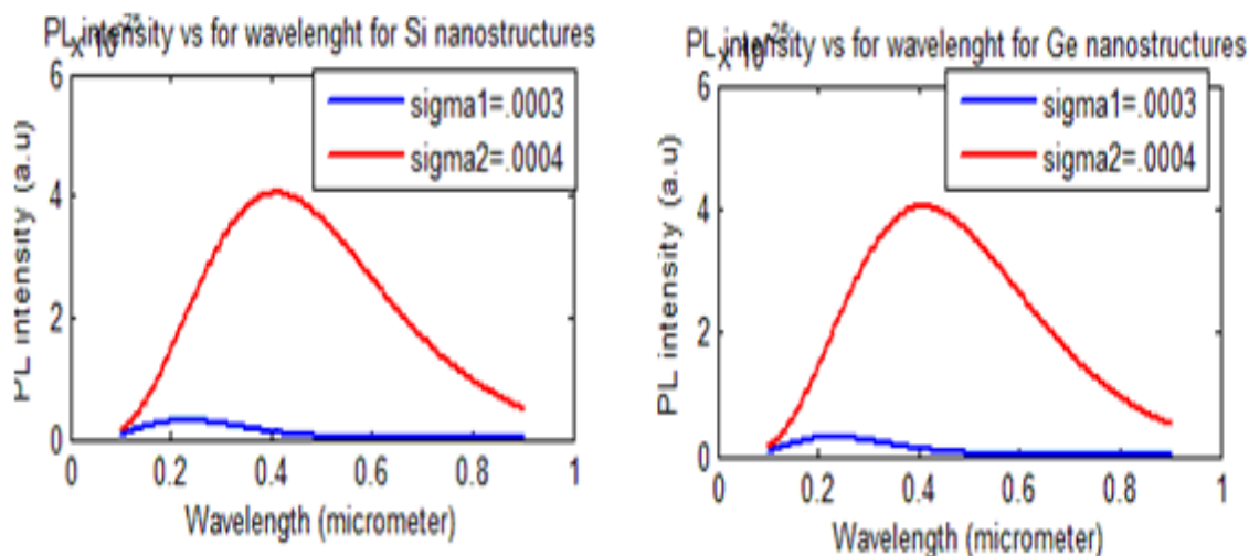
Figure 1: Dependence of PL intensity on wavelength: the left graph is for Si nanostructures and the right one for Ge nanostructures.
