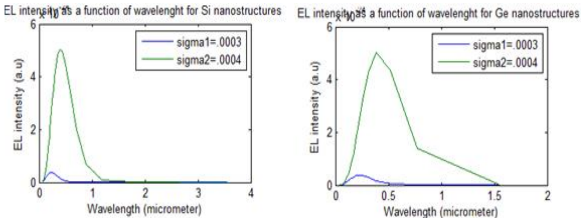
Figure 2: EL intensity as a function of wavelength: the left graph is for Si nanostructures and the right one for Ge nanostructures.
