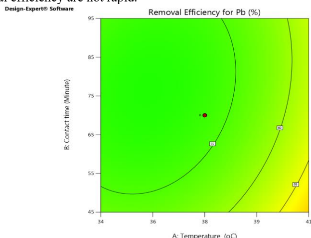
Figure 2: The contour plot showing the removal efficiency of RHBMO@500 for lead under the effect of temperature and contact time
