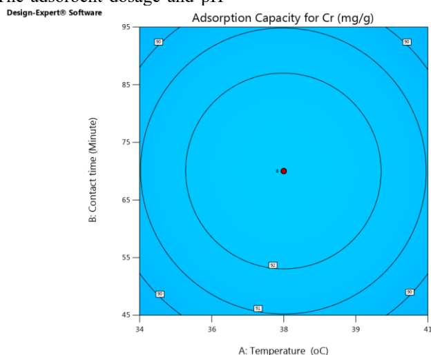
Figure 7: The contour plot showing the effect of temperature and contact time on the adsorption capacity of RHBMO@500 for chromium
