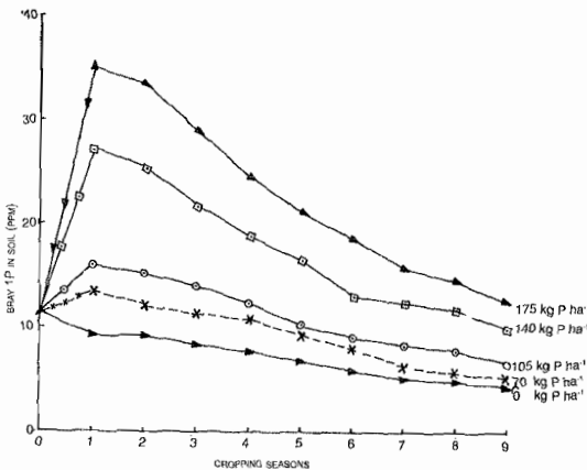
Fig. 1. Soil P test values as a function of time for broadcast P treatments on an Ultisol in Kumasi, Ghana
