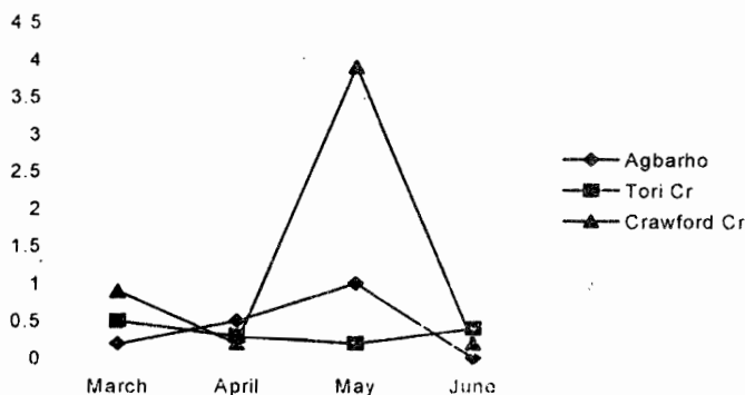
Fig. 2: Monthly and Spatial Variations in Surface Water PCBs Concentration in Warri River
