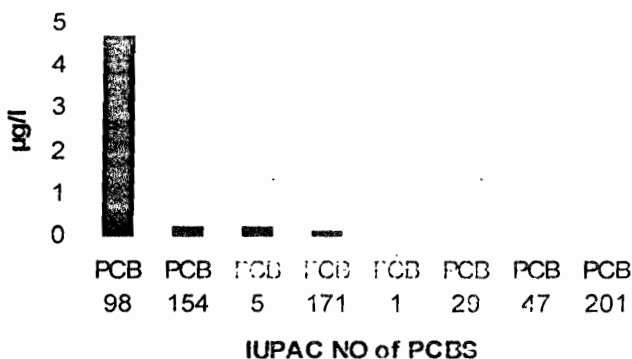
Fig. 5: Distribution of 8 individual Congeners in Surface Water from Warri River at Tori Creek Station
