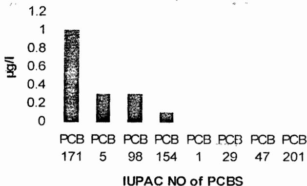
Fig. 4: Distribution of 8 individual Congeners in Surface Water from Warri River at Agbarho station
