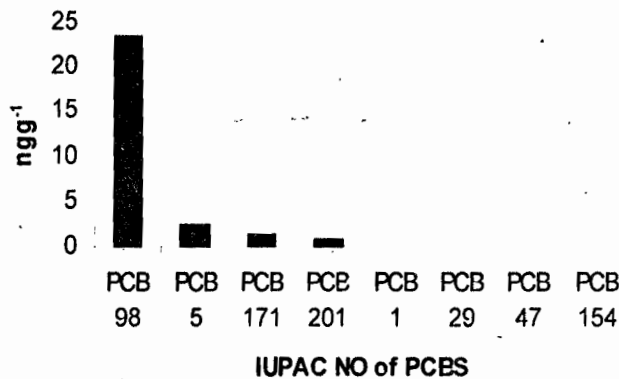
Fig. 9: Distribution of 8 individual Congeners in Sediment form Warri River at Crawford Creek Station
