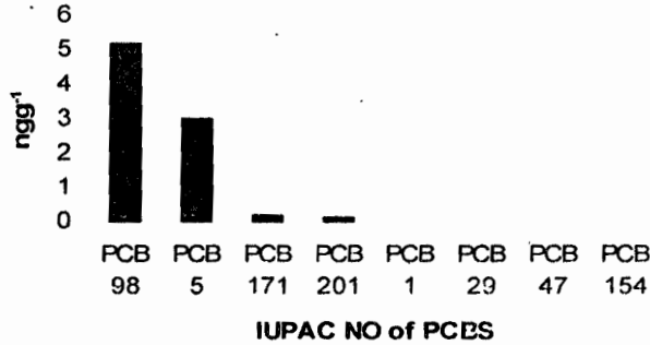
Fig. 7: Distribution of 8 individual congeners in Sediment form Warri River at Agbarho Station
