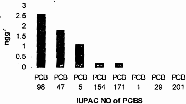
Fig. 8: Distribution of 8 individual congeners in Sediment form Warri River at Tori Creek Station
