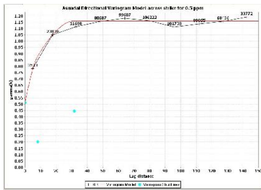
Fig. 9 Indicator Semi-variogram across Strike for 0.5 Cut-off
