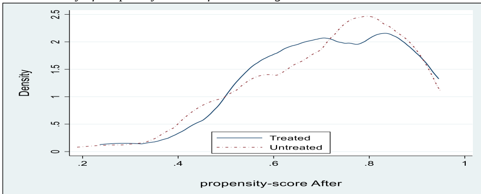
Figure 2: Kernel Density of Propensity Scores after Matching
