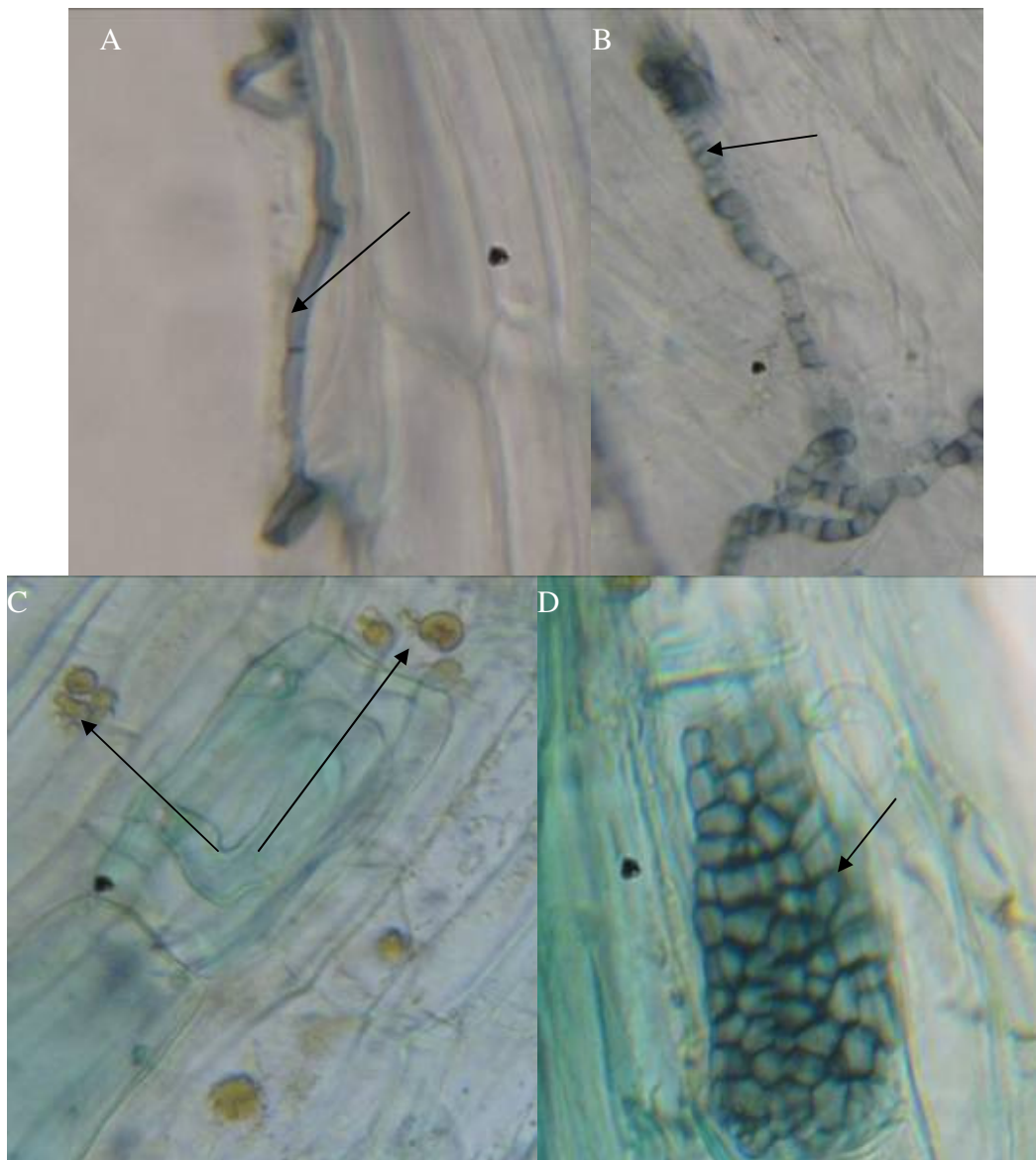
Fig.3: Mycorrhized roots of L. europaeum representing septate filaments (A) and kinds of encysted filaments (B) and other structures of endophytes (C et D) (G. \times 400 ).
