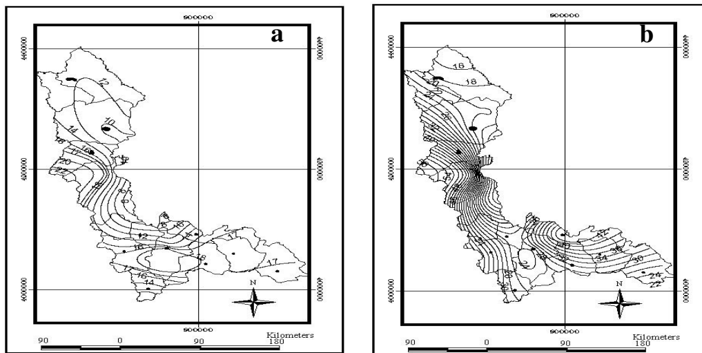
Fig 4. The map of the SPI with time scale 12-month and return period 5-year (a) and 25-year (b) during 1963-2003 in the West Azarbaijan province.
