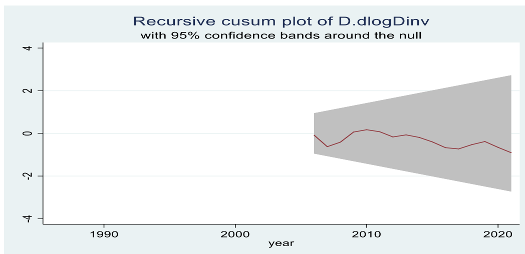
Figure 2: CUSUM plot
