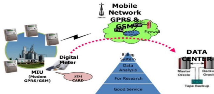
Fig.2. AMR system architecture [9]
