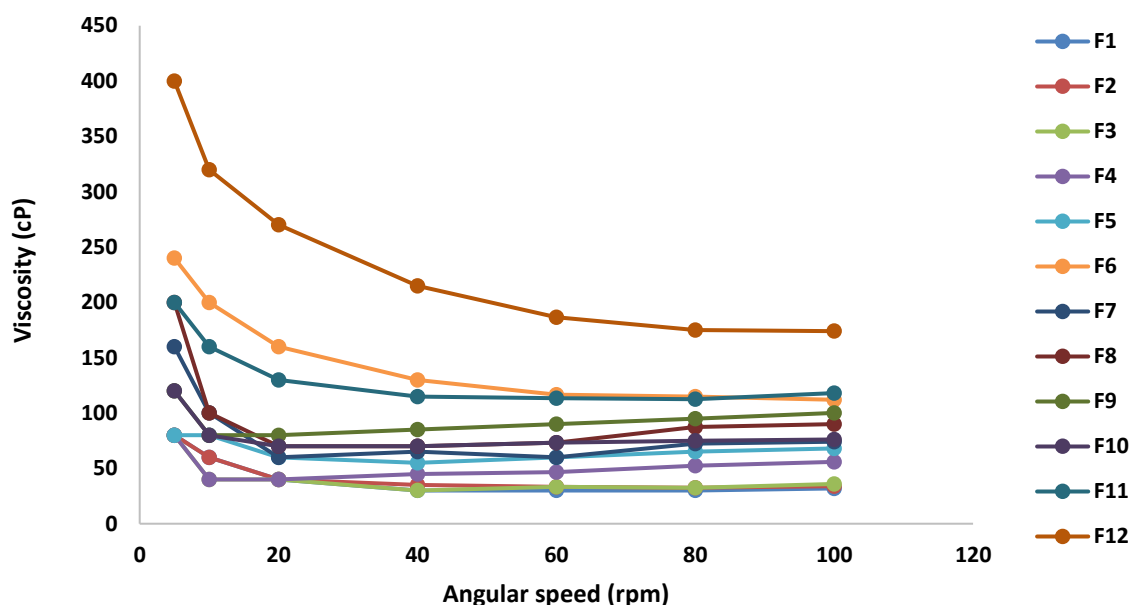
Figure 3: Formulations F1 – F12 rheograms of viscosity measurement against angular speed in revolutions per minute (rpm).
