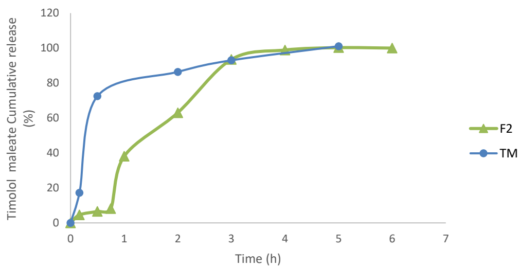
Figure 4: Percentage timolol maleate cumulative drug release from (a) Formulations F1 – F12 ISGs and TM solution (control) (b) Optimized ISG formulation, F2, and TM solution (control) release.
