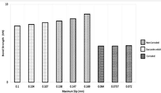
Figure 7: Bond strength versus maximum slip
