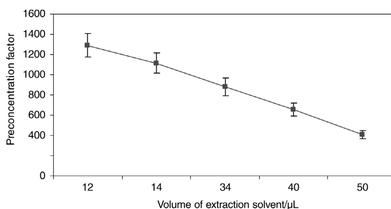
Figure 4 Effect of the extraction solvent volume on the preconcentration factor. Conditions: sample solution: 10 mL of 100 \mu\text{g L}^{-1} of the analyte without salt; volume of toluene: 12.0, 14.0, 34.0, 40.0 and 50.0 \mu\text{L} ; solution temperature: 25 \pm 3 \text{ }^\circ\text{C} ; dispersion time: 30 seconds; centrifugation time: 10 min ( n = 3 ).
