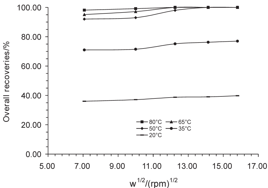
Figure 3 Dependence of the overall dissolution recoveries on the square root of the stirring speed at different temperatures.
