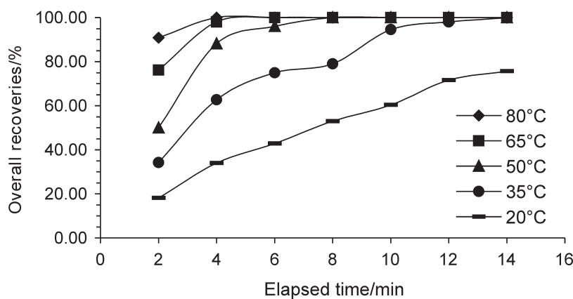
Figure 4 Dependence of dissolution recovery on the elapsed time at various temperatures.
