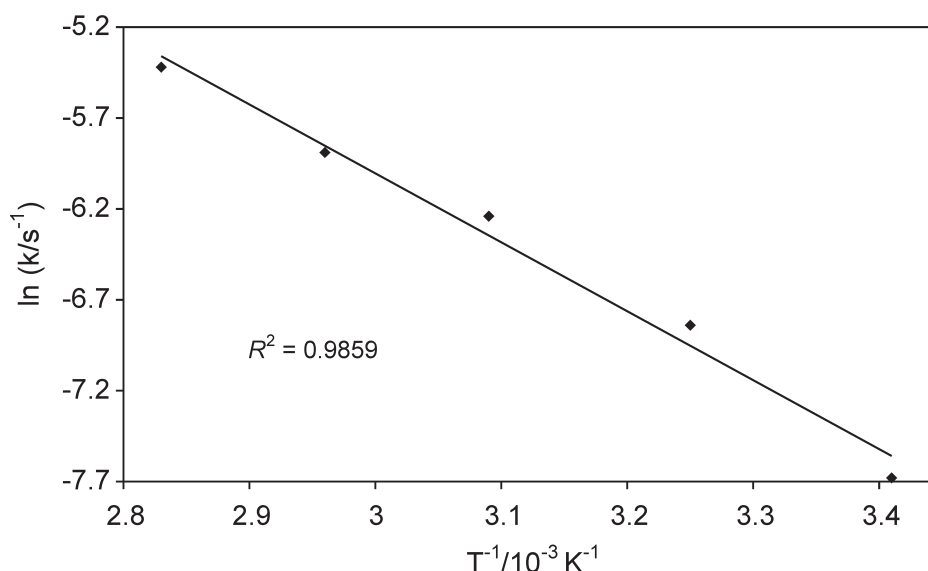
Figure 7 The Arrhenius curve obtained for the dissolution of the dolomite ore.
