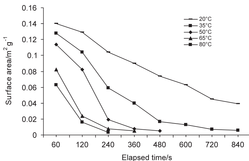
Figure 5 Final specific surface areas of the samples undissolved as a function of time at various temperatures.
