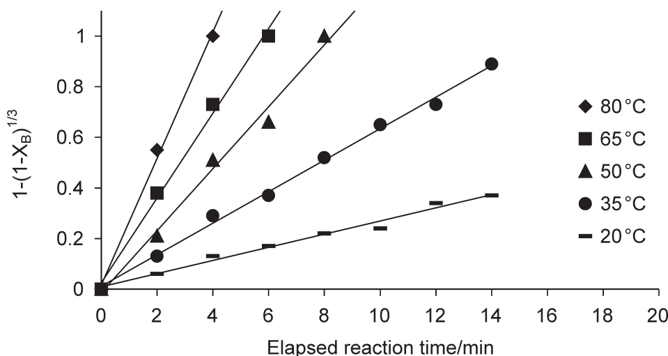
Figure 6 Plot of the dolomite dissolution data according to shrinking core model with surface reaction kinetics.
