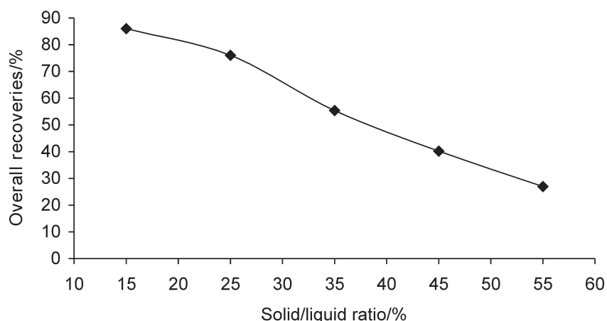
Figure 2 Effect of the solid/liquid ratio (m/v) on dissolution recoveries of the dolomite ore based on the mass losses.
