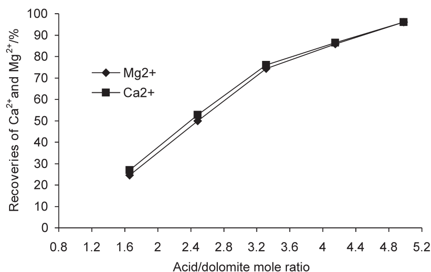
Figure 1 Effect of the acid-to-dolomite mole ratio on the extraction recoveries of Ca 2+ and Mg 2+ from the dolomite ore.
