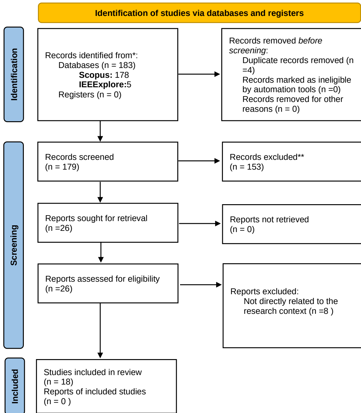
Figure 3. The PRISMA 2020 Flow Diagram of the Papers Selection Processes
