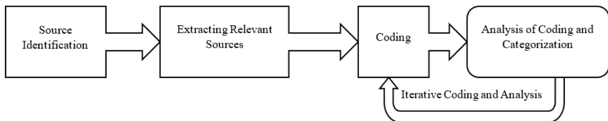
Figure 1. Outline of Research Process
