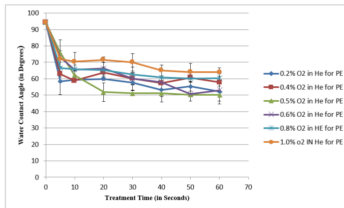
Fig. 2: Measured contact angle of PE film as a function of treatment time with the APPJ at various O 2 admixtures.
