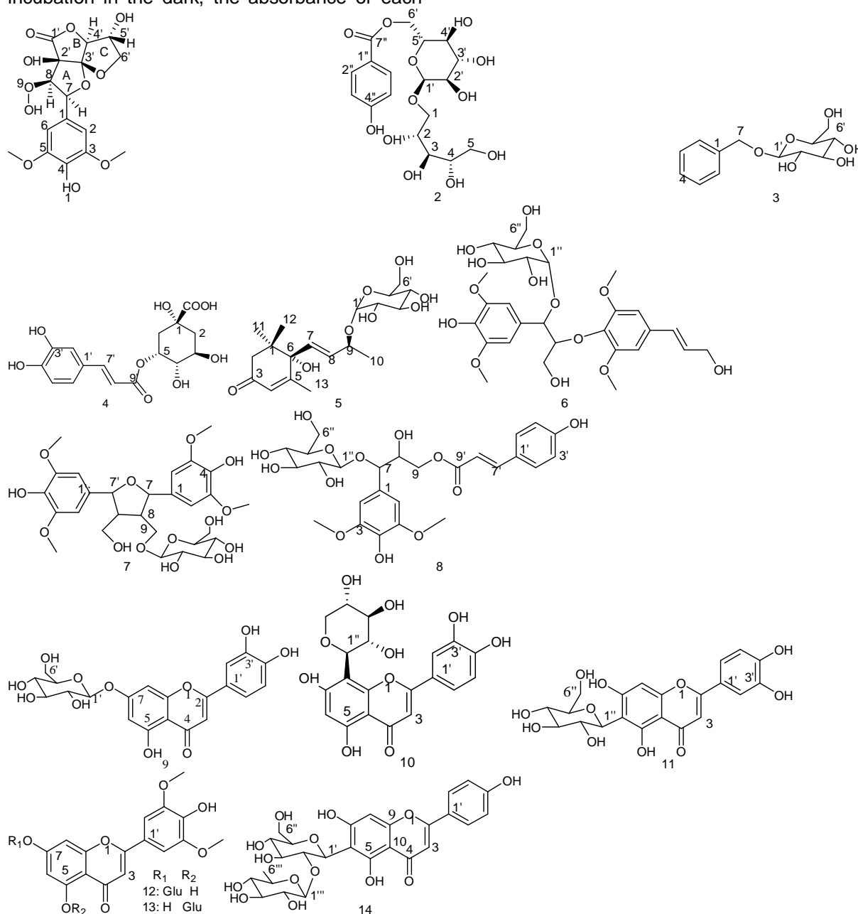
Figure 1: Structures of compounds (1-14) isolated from Phyllostachys prominens
