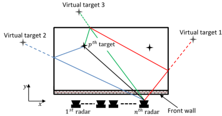
Figure 1: A multipath scenario with first-order returns.
