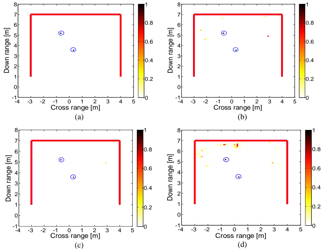
Figure 5: Image reconstruction (a) original scene, (b) Duo-subarray final image, (c) Hybrid final image, and (d) Pythagorean-based displaced subarray.
