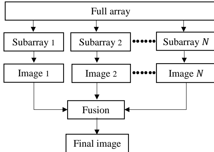
Figure 2: Multiple subarrays image formation.
