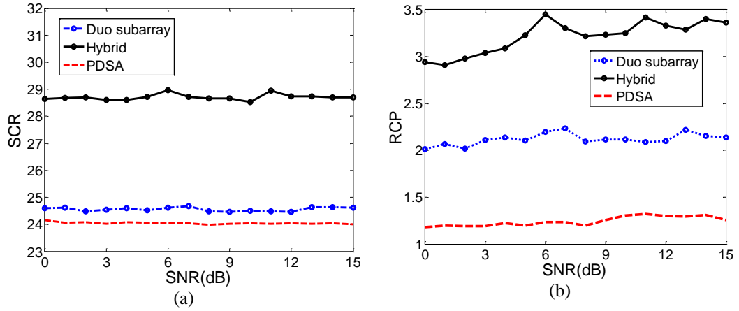
Figure 6: Performance metrics at different SNR: (a) SCR, and (b) RCP.
