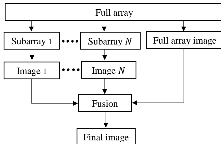
Figure 3 : Hybrid subarray image formation.
