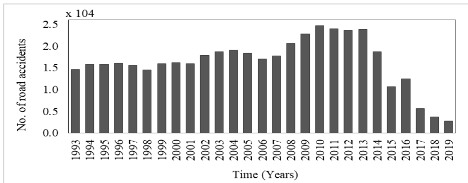
Figure 1: Histogram for road accidents data.
