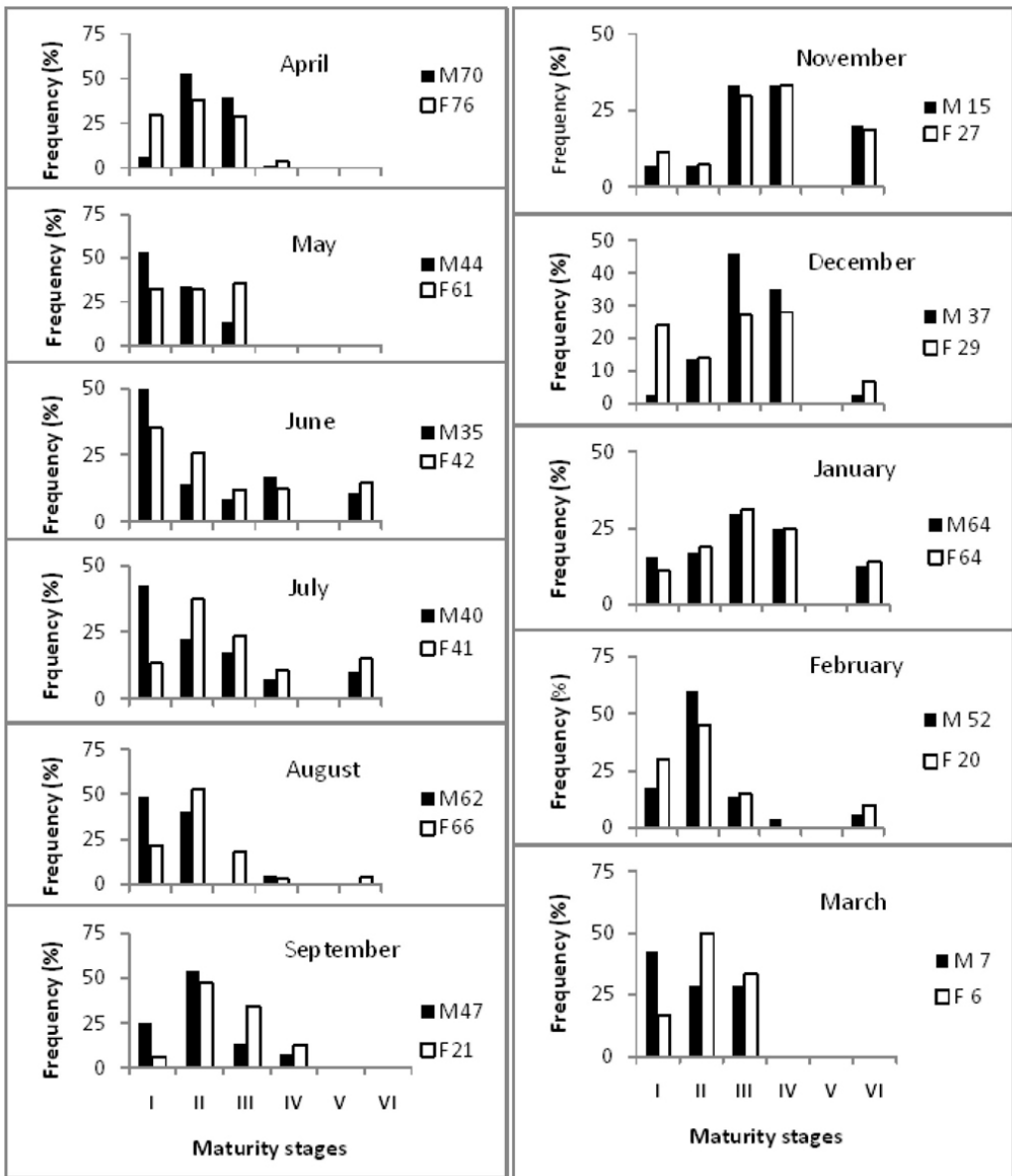
Figure 6. Distribution of monthly maturity stages of Siganus canaliculatus gonads during 2005-2007 in the Arabian Sea coast of Oman (pooled data).
