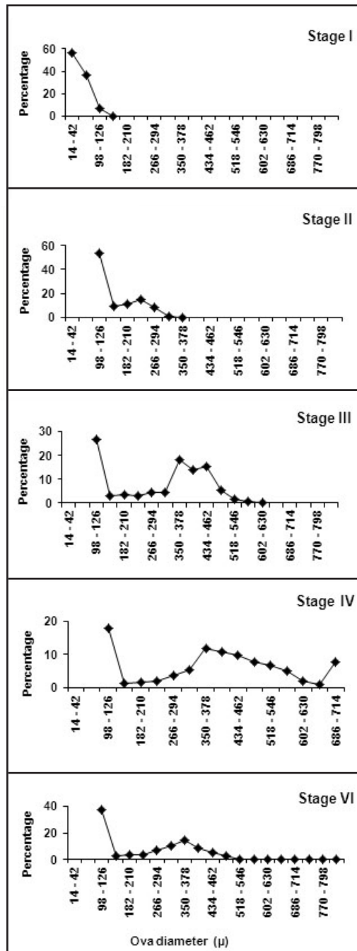
Figure 2. Development of ova to maturity in Siganus canaliculatus in the Arabian Sea coast of Oman.
