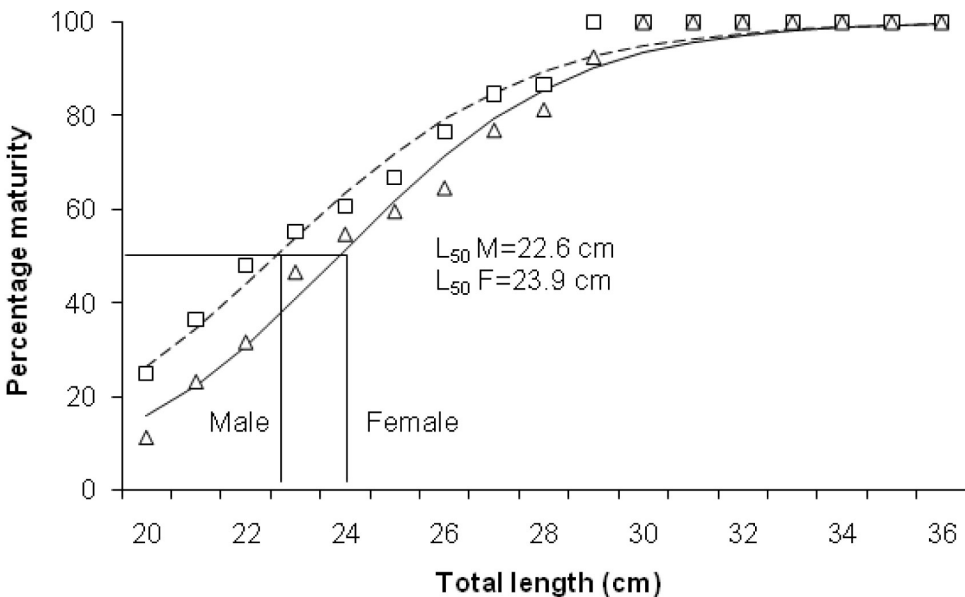
Figure 5. Size at first maturity of Siganus canaliculatus in the Arabian Sea coast of Oman.
