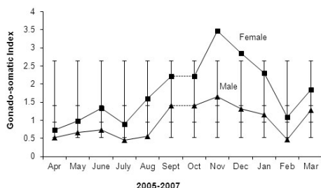
Figure 3. Gonado-somatic indices in Siganus canaliculatus during 2005-2007 in the Arabian Sea coast of Oman.
