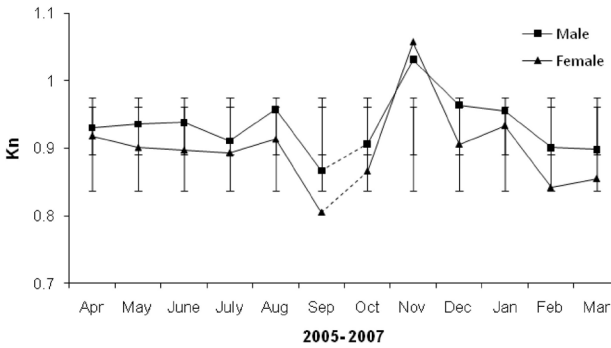
Figure 4. Monthly relative condition factors (Kn) of Siganus canaliculatus during 2005-2007 in the Arabian Sea coast of Oman.
