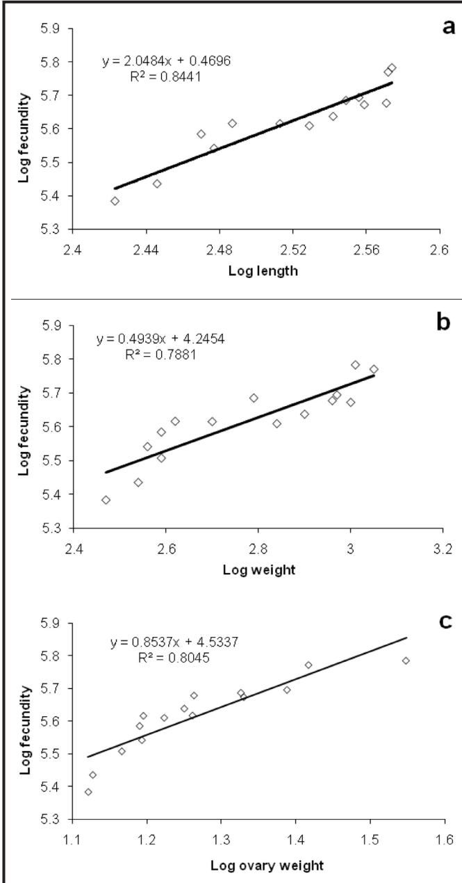
Figure 7. Fecundity of Siganus canaliculatus relative to a) total length b) body weight and c) ovary weight in the Arabian Sea coast of Oman.
