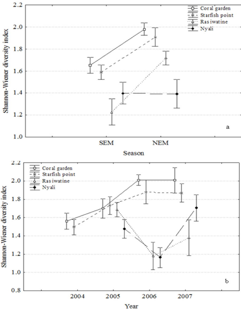
Figure 6. Mean ± SE Shannon-Wiener indices of fish diversity at the sampling stations in a) seasons and b) years.
